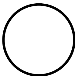
Mars Yellowish-white
